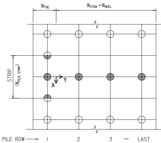
PILE LAYOUT
